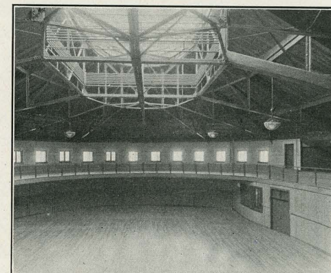
William Hall Walker Gymnasium—Main Floor and Running Track
