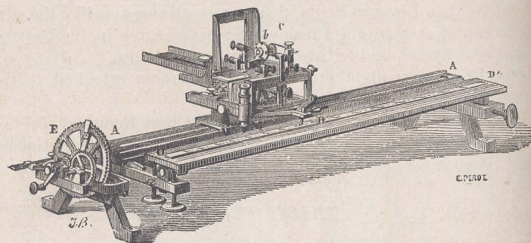
DIVIDING ENGINE. BY J. SALLERON.
